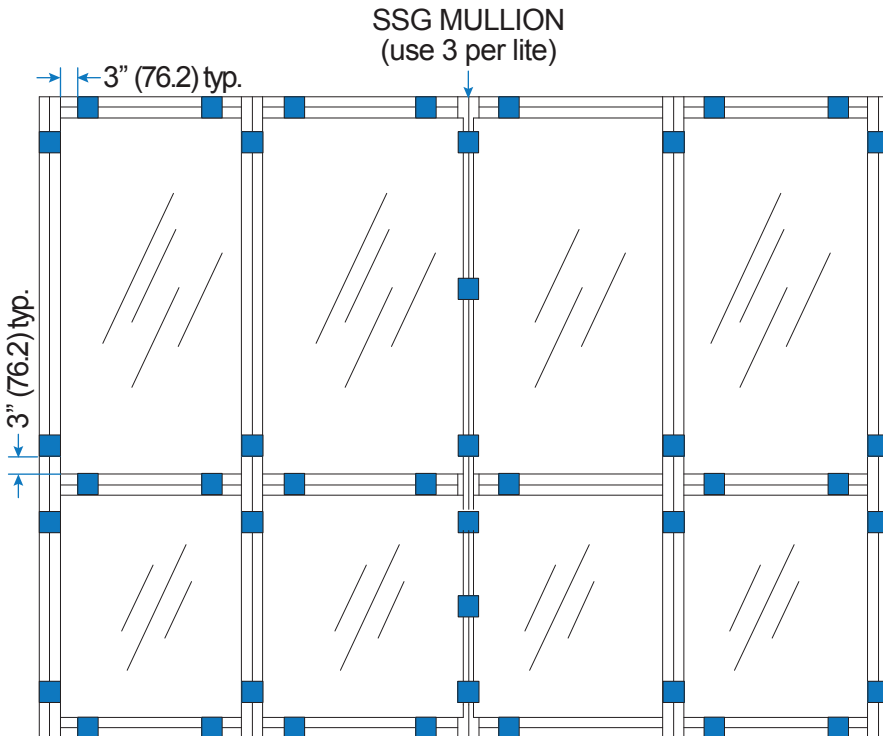
Typical Temporary Glazing Retainer Location
